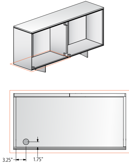
2" Grommet in Bottom Panel Cutout
