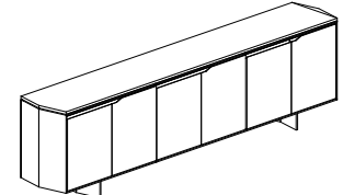
Beveled Case 108"/111.5" L x 18" D x 30" H 108"/112.75" L x 24.5" D x 30" H
