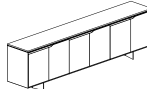
Standard Case 108" L x 18" D x 30" H 108" L x 24.5" D x 30" H
