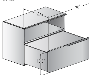
Center Box / Large Box Drawer O51LD
