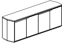
Beveled Case 72"/75.5" L x 18" D x 25" H 72"/76.75" L x 24.5" D x 25" H
